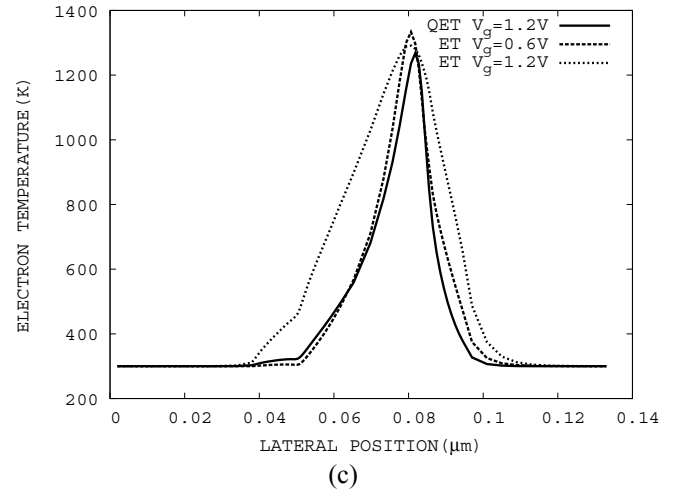
Fig.4 Lateral profiles of electron temperature distributions calculated by QET(solid line) and ET(dotted line) models at the same drain bias of V_d=0.8V . (a) QET model at V_g=0.3V , ET model at V_g=0.3V and V_g=0.2V . (b) QET model at V_g=0.8V , ET model at V_g=0.8V and V_g=0.5V . (c) QET model at V_g=1.2V , ET model at V_g=1.2V and V_g=0.6V .
